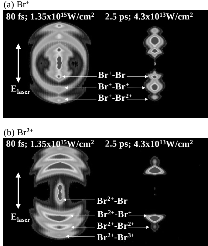
Figure 4.2: Experimental images of \text{Br}^+ (a) and \text{Br}^{2+} (b) fragments resulting from the multi-electron dissociative ionization (MEDI) of \text{Br}_2 for short and long laser pulses. The pulse durations and intensities are indicated in the figure. The laser polarization is along the vertical axis.
