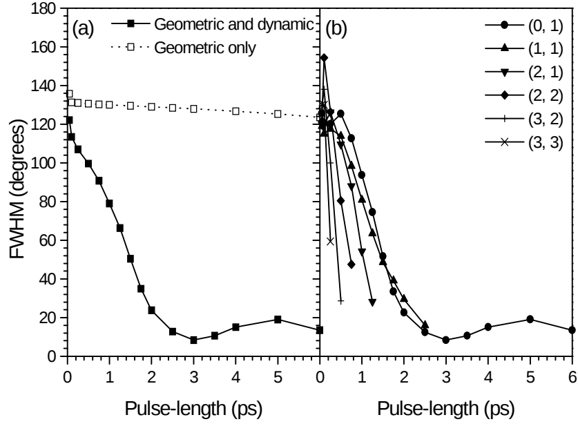
Figure 5.7: FWHM with pulse duration at fixed fluence of 100 \text{ Jcm}^{-2} . (a) For all ions at fluences of 100 \text{ Jcm}^{-2} with both geometric and dynamic alignment (solid lines, filled squares) and with geometric alignment alone (dotted lines, open squares). (b) For each charge channel from (0, 1) to (3, 3).
