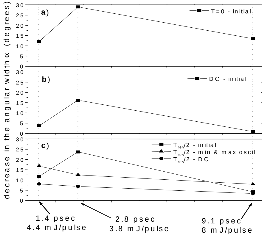
Figure 6.14: The decrease in the angular width \alpha of the I^{2+} fragments from the I^{2+} - I^+ channel for: (a) the maximum alignment at \Delta t = 0 , (b) the amplitude of the half revival and (c) the residual alignment as a function of the pump pulse duration. This results are based on the measurements shown in Fig. 6.13.
