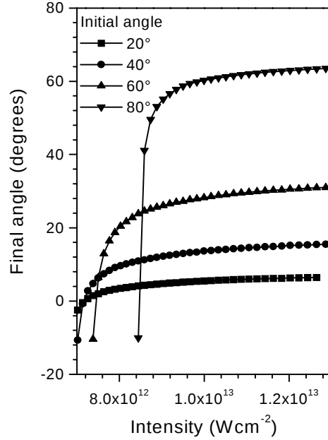
Figure 5.5: Final angles reached by molecules with initial angles of 20^\circ (squares), 40^\circ (circles), 60^\circ (up triangles) and 80^\circ (down triangles) as a function of laser intensity. For each data point plotted, the laser pulse was 1500 fs long and the charge channel reached was (0, 1).
