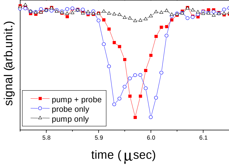
Figure 6.6: Time-of-flight measurement of I_2^+ fragments. The shape of the peaks is used to optimize the spatial and temporal overlap between the pump and the probe lasers. The probe only signal contains two peaks corresponding to the backward and forward ejection of fragments with respect to the detector (circles). The pump laser alone gives almost no signal (up triangle). The pump + probe signal has only one contribution corresponding to molecules aligned by the pump laser in the plane of the detector (squares).
