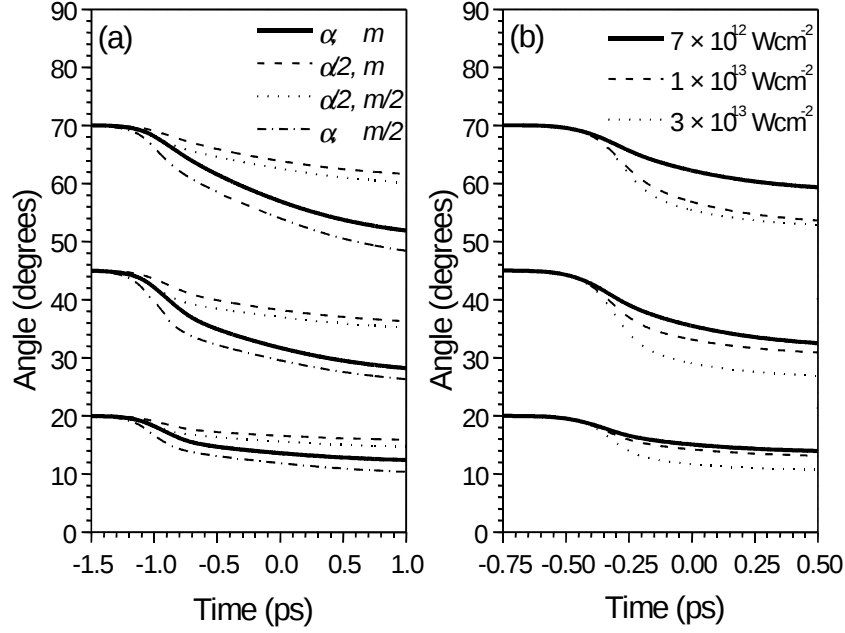
Figure 5.8: Trajectories for ions with 3 different initial angles ( 20^\circ , 45^\circ and 70^\circ ) for 500fs laser pulses with a peak intensity of 2 \times 10^{14} \text{ Wcm}^{-2} . (a) Mass or polarizability changed. Thick solid lines: iodine ions ( \alpha = \alpha_{\text{iodine}} = 45.146 \text{ au} , m = m_{\text{iodine}} = 126.9 ). Dashed lines: \alpha = \alpha_{\text{iodine}}/2 . Dash-dotted lines: m = m_{\text{iodine}}/2 . Dotted lines: \alpha = \alpha_{\text{iodine}}/2 , m = m_{\text{iodine}}/2 . (b) Trajectories with 3 different threshold intensities: 7 \times 10^{12} , 1 \times 10^{13} and 3 \times 10^{13} \text{ Wcm}^{-2} .
