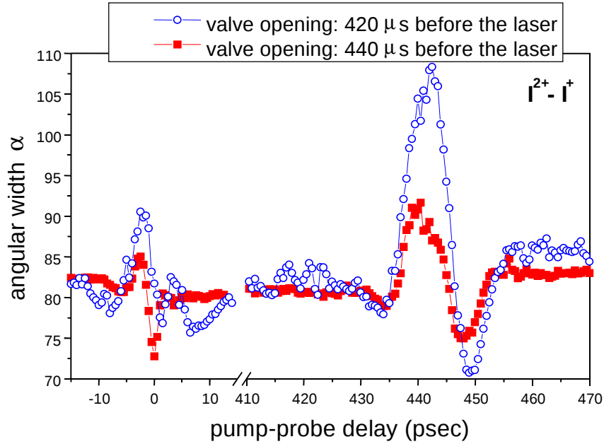
Figure 6.15: The time evolution of the angular width of the I^{2+} fragments from the I^{2+} - I^{+} channel as a function of the opening time of the valve: 420 \mu\text{sec} before the laser (circles), 440 \mu\text{sec} before the laser (squares). The time-dependent angular width \alpha is shown both around \Delta t = 0 and around the full revival. The pump pulse energy and pulse duration were \sim 3\text{mJ/pulse} and 1.4\text{psec} , and the probe pulse energy and pulse duration were \sim 1\text{mJ/pulse} and 100\text{fsec} . The backing pressure was 1.2\text{bar} .
