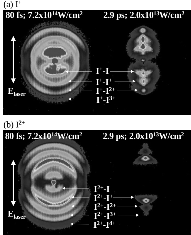
Figure 4.1: Experimental images of I^+ (a) and I_2^+ (b) fragments resulting from the multi-electron dissociative ionization (MEDI) of I_2 for short and long laser pulses. The pulse durations and intensities are indicated in the figure. The laser polarization is along the vertical axis in the plane of the image.
