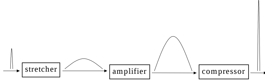
Figure 2.1: The amplification of ultrashort pulses is done using a technique called "Chirped Pulse Amplification". As the name suggests, in this technique the short pulse is first chirped (stretched in time), then amplified and in the end of the laser system compressed back to its original duration.
