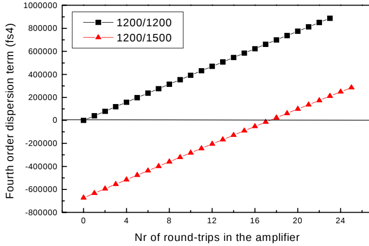
Figure 2.4: Dispersion compensation in the amplifier for different gratings combination in the stretcher and in the compressor. The fourth-order dispersion term is minimized for a combination of 1200lines/mm groove density in the stretcher and 1500lines/mm groove density in the compressor.
