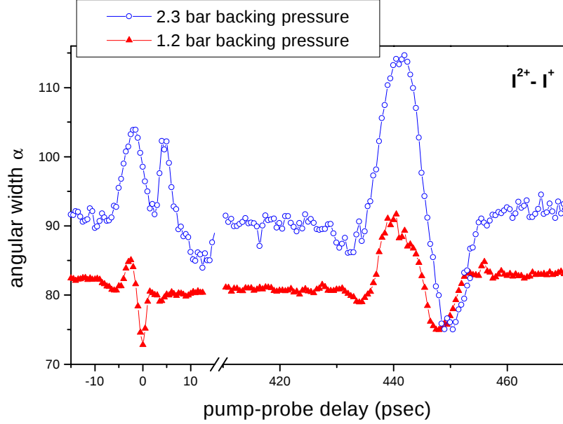
Figure 6.16: The time evolution of the angular width for I^{2+} fragments from the I^{2+} - I^{+} channel for backing pressures of 2.3 bar (circles) and 1.2 bar (up triangles). The time-dependent angular width is shown both around \Delta t = 0 and around the full revival. The valve was opened 440\mu s before the lasers. The pump pulse energy and pulse duration were \sim 2mJ/pulse and 1.4psec , and the probe pulse energy and pulse duration were \sim 0.5mJ/pulse and 100fsec .
