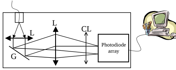
Figure 2.21: Overview of the Optical Multichannel Analyzer (OMA). The beam is coupled into a fiber which represents a point source for a 8cm focal length lens that collimates the beam. The collimated beam is diffracted by a grating with a groove density of 600lines/mm. The diffracted beam is focused by another 8cm focal length lens onto a photodiode array which gives the pulse spectrum. L = lens, G = grating, CL = cylindrical lens.
