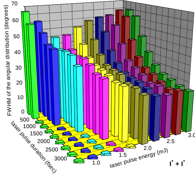
Figure 4.6: The FWHM of the angular distribution versus the laser pulse duration and laser pulse energy for the I^+ signal resulting from the I^+-I^+ channel formed in the Coulomb explosion of I_2 . The FWHM are calculated by a gaussian fit of the experimental angular distribution after the inversion, as shown in Fig.4.3. The pulse duration is given in fs and the pulse energy is given in mJ. Based on a calibration of the absolute intensity using ATI in Xe, the intensity in the measurement is equal to (2.65 \times 10^{16}) E(mJ)/\Delta t(fs) W/cm^2 .
