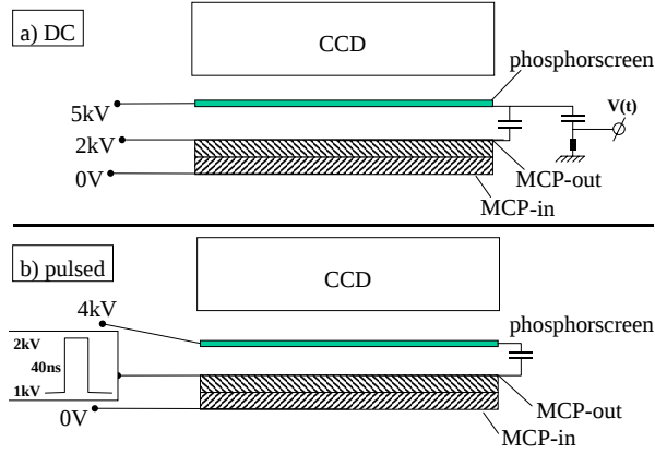
Figure 3.7: Two ways of using the MCP/phosphor-assembly: a) DC-mode: MCP-out is at \sim 2\text{kV} and the phosphorscreen at \sim 5\text{kV} . The charge collection as a function of time can be measured as a DC-signal V(t) using the simplified circuit shown in the figure. b) Pulsed mode: The phosphorscreen is at 4\text{kV} and the MCP is at 1\text{kV} , resulting in very low gain. To select a window in the time-of-flight spectrum, at a certain time the MCP-out is pulsed to \sim 2\text{kV} for \sim 150\text{ns} . Because of the capacitor the voltage difference between MCP-out and phosphor remains at 3\text{kV} .
