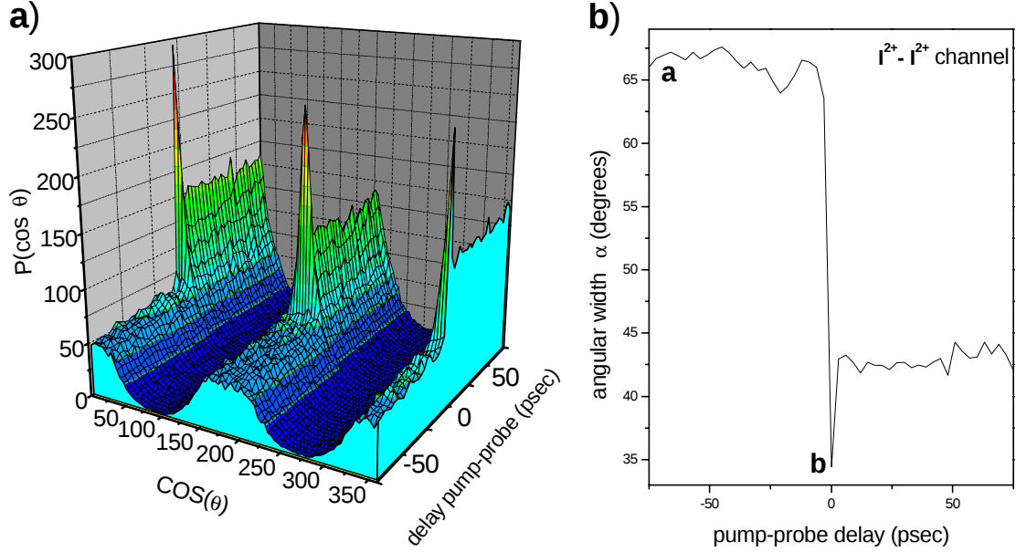
Figure 6.7: The time-evolution of the angular distribution of the \text{I}^{2+} - \text{I}^{2+} channel is shown by plotting (a) the angular distribution or (b) the angular width \alpha as a function of the time delay between the pump (2.2 mJ pulse energy and 4.2 psec pulse duration) and the probe (1 mJ pulse energy and 100 fsec pulse duration). The polarization of the two lasers is parallel to each other and parallel to the detector. Labels a and b given in the right graph refer to measurements shown in Fig 6.4.
