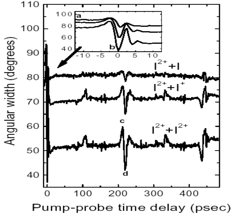
Figure 6.8: Pump-probe time delay scan, showing the angular width \alpha of the I^{2+} - I , the I^{2+} - I^+ and the I^{2+} - I^{2+} channels, recorded using a 3.8mJ 2.8 psec pump pulse polarized parallel to the plane of the imaging detector and a 1.2mJ 100 fsec probe pulse polarized perpendicular to the plane of the imaging detector. The measurements show alignment of the molecule during the pump laser pulse (see inset), residual alignment at the end of the pump laser pulse and the occurrence of rotational revivals. The labels (a)-(d) refer to the measurements shown in Fig. 6.5.
