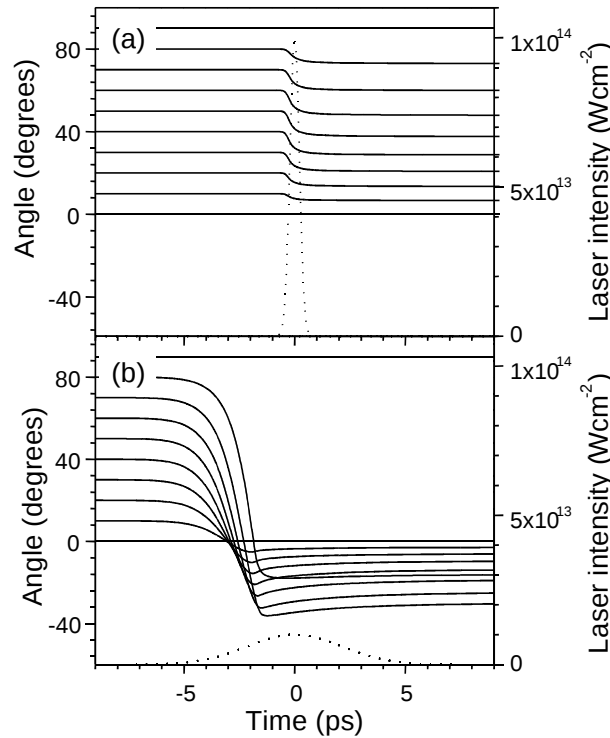
Figure 5.3: Calculated trajectories for ions with a range of initial angles for, (a), a 500 fs pulse with a peak intensity of 1 \times 10^{14} \text{ W cm}^{-2} and, (b), a 5 ps pulse with peak intensity 1 \times 10^{13} \text{ W cm}^{-2} . The dotted curves show the intensity of the laser pulse.
