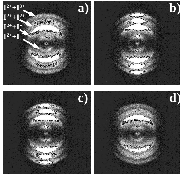
Figure 6.4: Raw I^{2+} images, recorded with a 4.2 psec 2.2mJoule pump laser (polarized parallel to the plane of the imaging detector along the vertical axis of the image) and a 100 fsec 0.9mJ probe laser (polarized parallel to the imaging detector); a) with the probe before the pump laser, b) with the pump and probe lasers overlapped in time, c) with the pump laser preceding the probe laser by 219 psec, d) with the pump laser preceding the probe laser by 225 psec.
