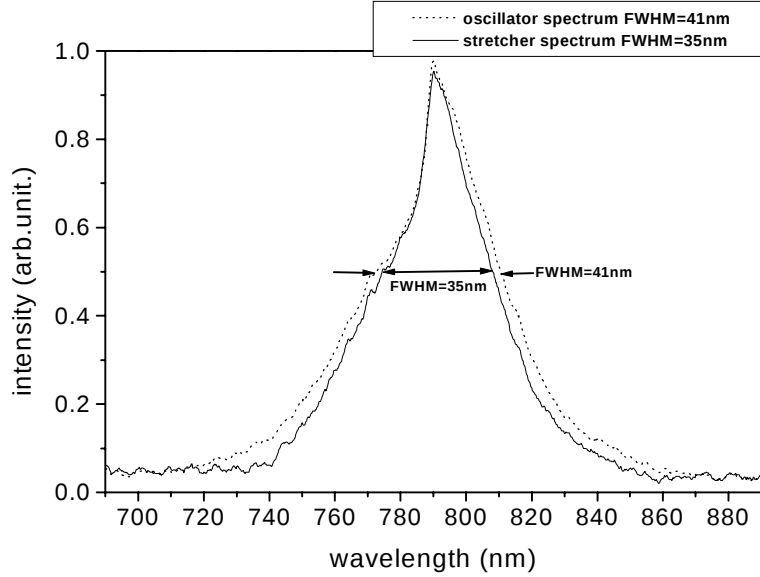
Figure 2.12: Spectrum of the laser pulse before and after the stretcher. The spectrum is narrower than the input spectrum due to the wavelength-dependent reflectivity of the stretcher grating.
